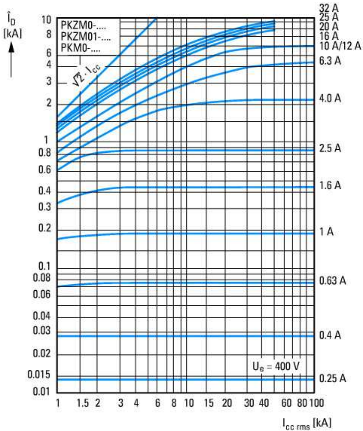
Let-through current
